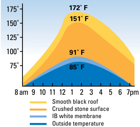
Heat Gain Comparison Chart
